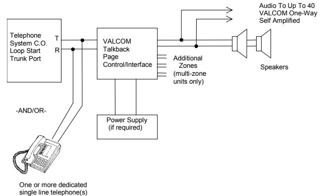
Block Diagram of Loop Start Trunk Port And/Or Single Line Telephone Access of a Valcom Talkback Page Control/Interface
